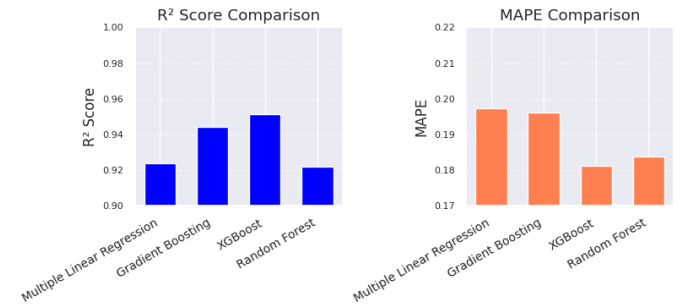
Fig. 6. Comparison of model performance
